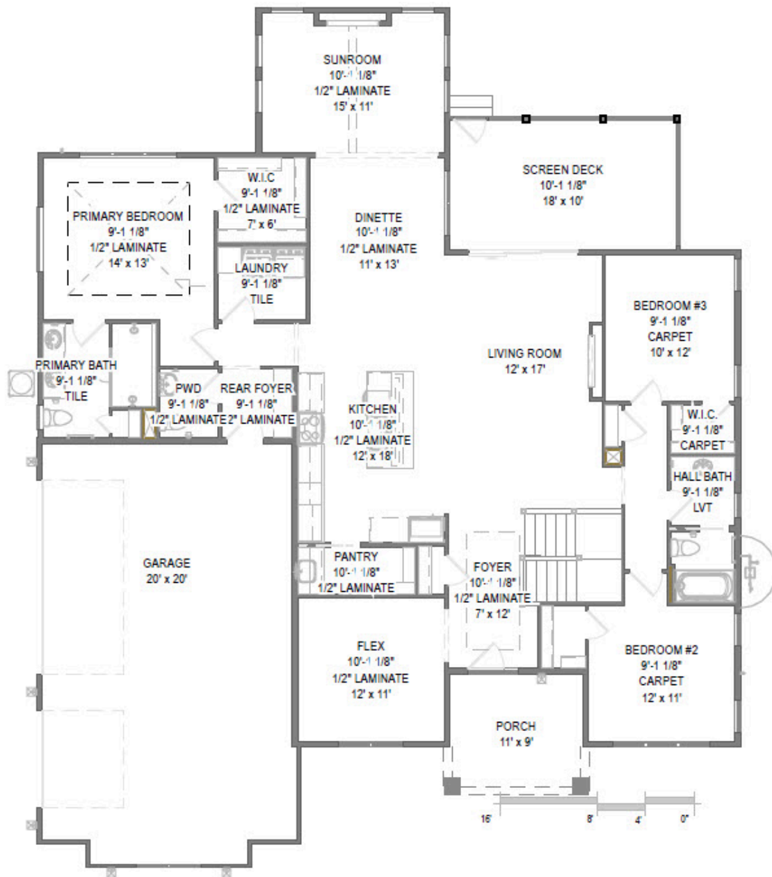
First Floor
