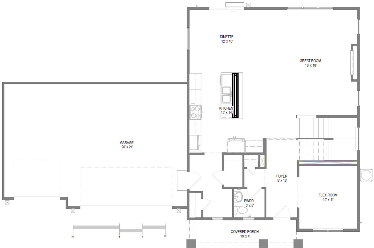
First Floor
