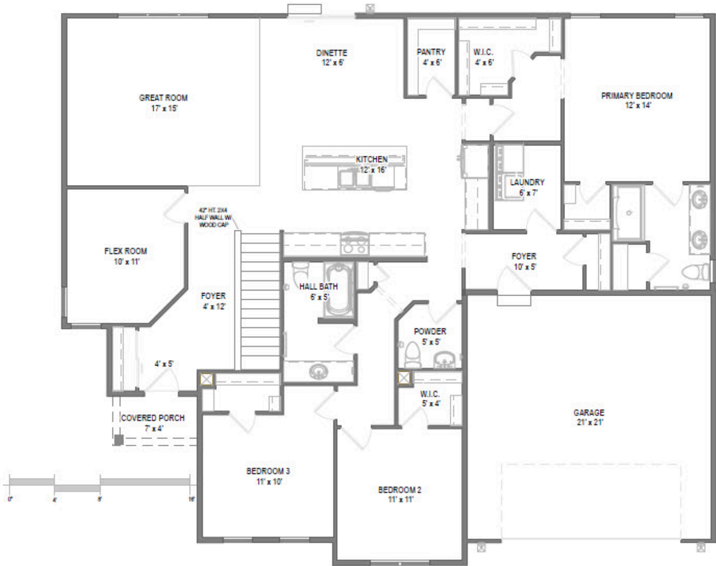
First Floor
