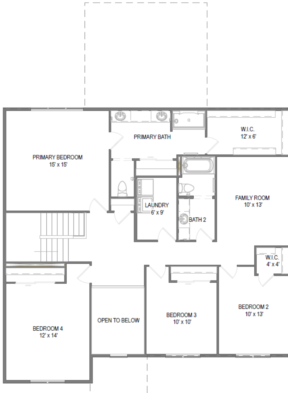
Second Floor
